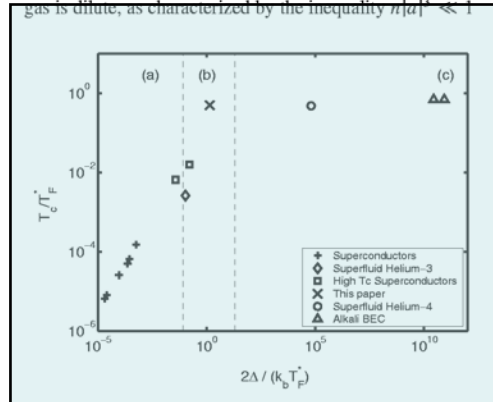
FIG. 1. A log-log plot showing six distinct regimes for quantum fluids. The transition temperature T_c is shown as a function of the relevant gap energy 2\Delta . Both quantities are normalized by an effective Fermi temperature T_F^* . For the BCS systems in region (a), and the systems in the crossover region (b), 2\Delta is the energy needed to break up a fermion pair, and T_F^* is the Fermi energy. For the systems in region (c), which are all strongly bound composite bosons and exhibit BEC phenomenology, 2\Delta is the smallest energy needed to break the composite boson up into two fermions, i.e., ionization to a charged atomic core and an electron, and T_F^* is the ionic Fermi temperature.
