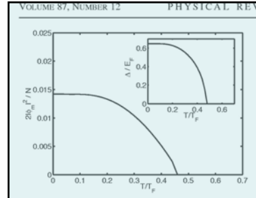
FIG. 3. The temperature at the phase transition is also visible from the amplitude of the molecular field. This amplitude is nonzero only when the broken symmetry exists in the region T < T_c . For T = 0 , the molecules form a Bose condensed fraction of 1.5% of the total gas sample. The inset shows the behavior of the gap \Delta = U\rho - g\phi_m . The critical temperature T_c can be related to the value of the gap at T = 0 . For comparison, in superconductors the analogous gap is simply the binding energy of a fermion pair.
