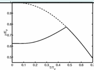
FIG. 2. Chemical potential as a function of temperature for the system of resonance pairing (solid line). The second-order phase transition occurs at T_c \approx 0.5T_F where a clear gap is visible. The dashed line shows the chemical potential of a noninteracting Fermi gas.
